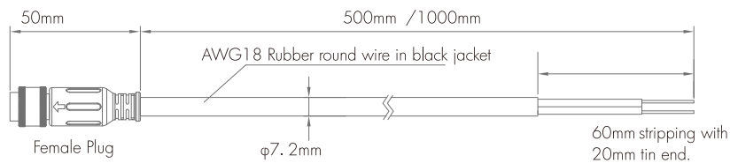
F3-RL-PC2 / F3-RL-PC5
