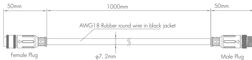
F3-RL-EX2 / F3-RL-EX5
