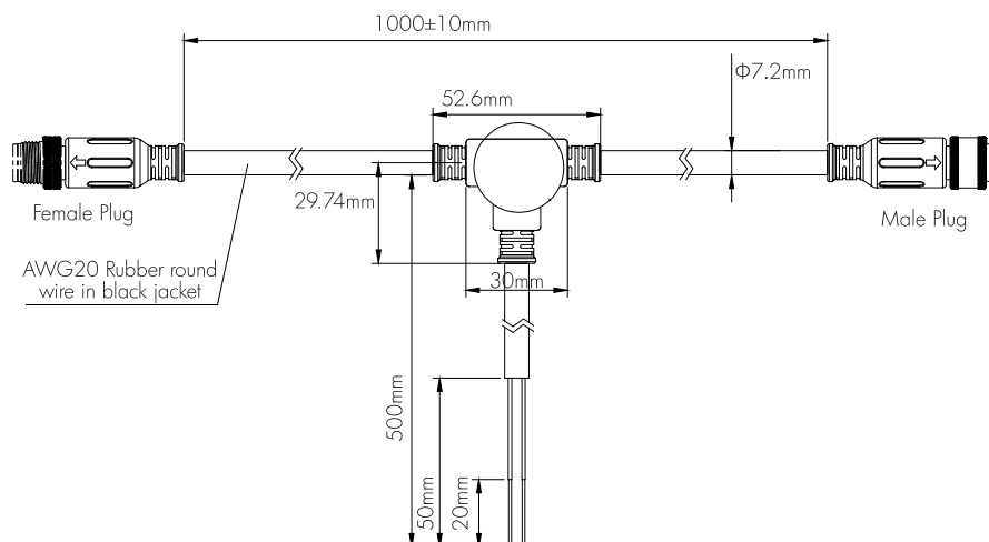
F3-RL-TC2 / F3-RL-TC5
