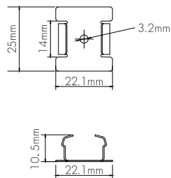
F3-RL-SM
