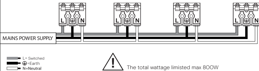
Loop in & Loop out wiring diagram
