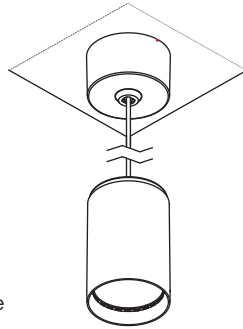
6 - Finish installation
