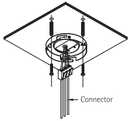
4 - Connect the AC power to the connectors
