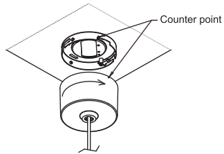
5 - Align the driver box to the counterpoint and rotate clock wise to fix onto the back base
