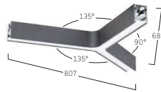
Y3-Junction
