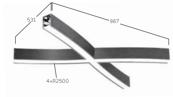
X2-Junction Module
