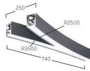
Y1-Junction
