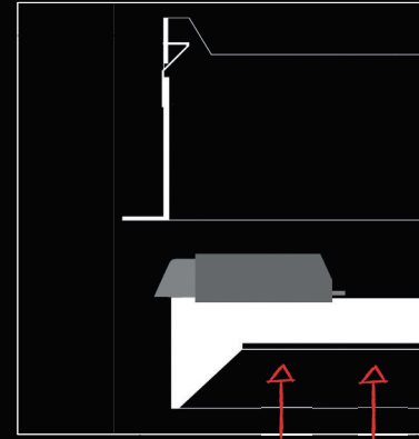
STEP 3 BELA FIXED (mounting device fixes the luminaire)
