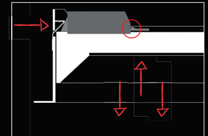
STEP 4 DEMONTAGE - push in luminaire (mounting device pushes back and fixes itself in place)
