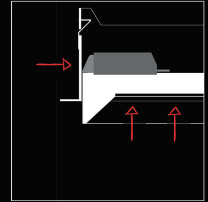
STEP 4 DEMONTAGE - push in luminaire (mounting device pushes back and fixes itself in place)
