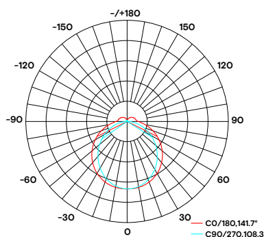
BEAM ANGLE 122°
