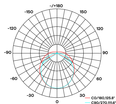
BEAM ANGLE 150°
