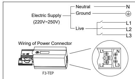
Track circuit wiring diagram
