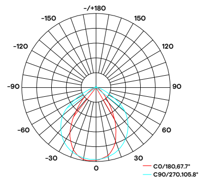
BEAM ANGLE 60°
