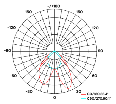
DOUBLE ASYMMETRIC 30°
