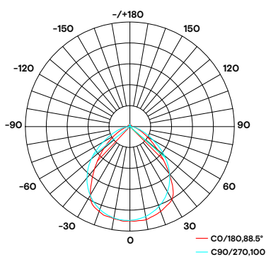
BEAM ANGLE 90°
