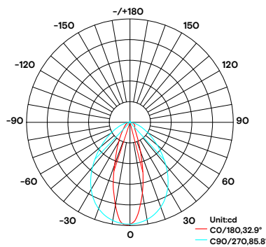
BEAM ANGLE 30°
