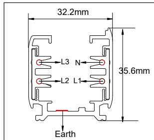
Track Technical Drawing
