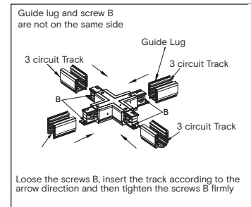
X Connector
