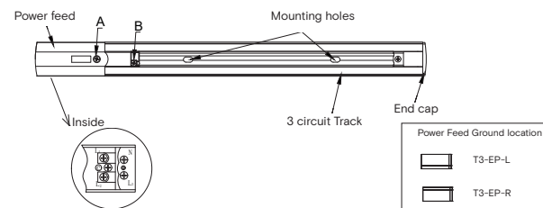
General track connection
